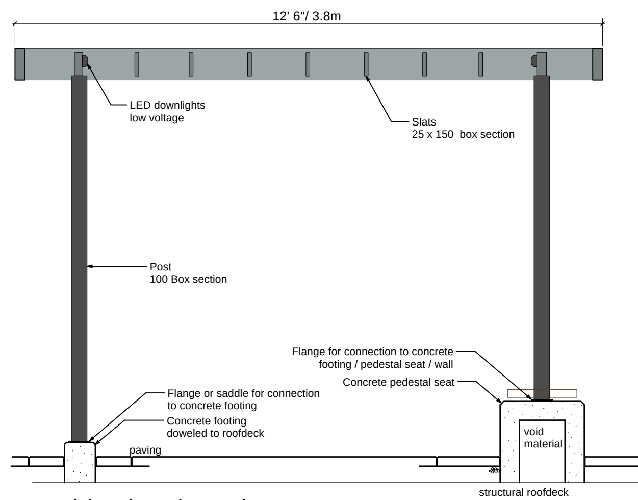
Side view / Section
