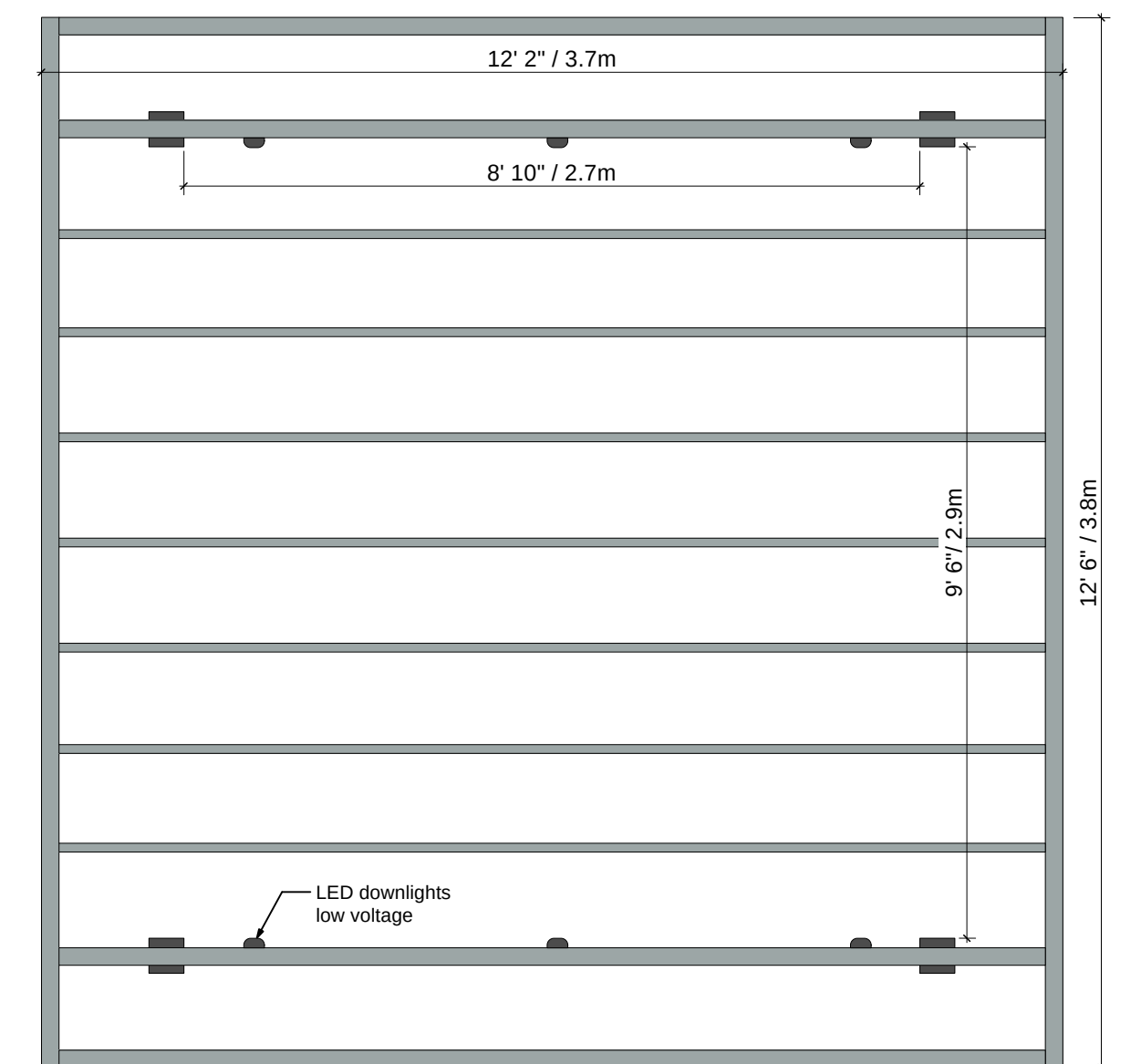
Plan view
