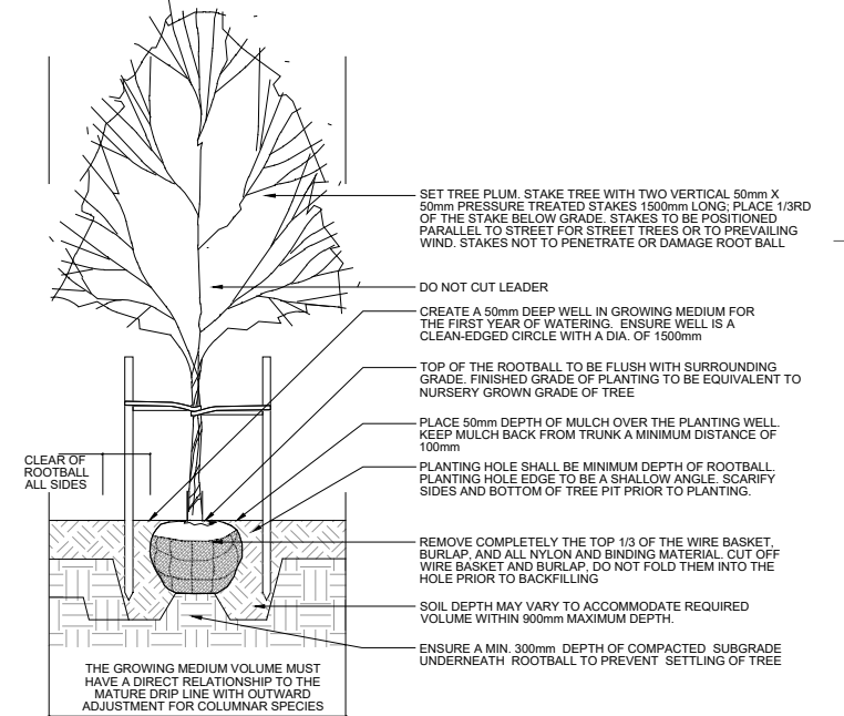
3 TREE PLANTING SCALE: NTS
