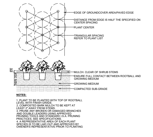
1 GROUND COVER PLANTING SCALE: NTS
