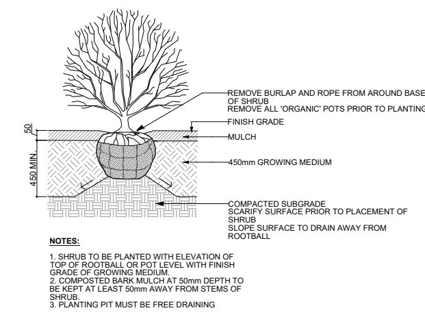
2 SHRUB PLANTING SCALE: NTS
